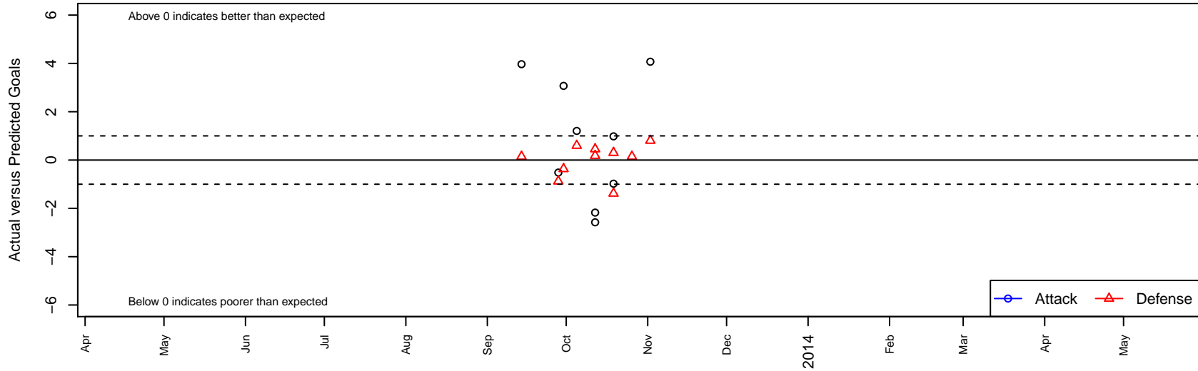
SSC Shadow Dempsey B02 Dots are actual minus expected GF (blue circles) and GA (red triangles). Blue line is smoothed change in attack strength. Red is smoothed change in defense strength.
